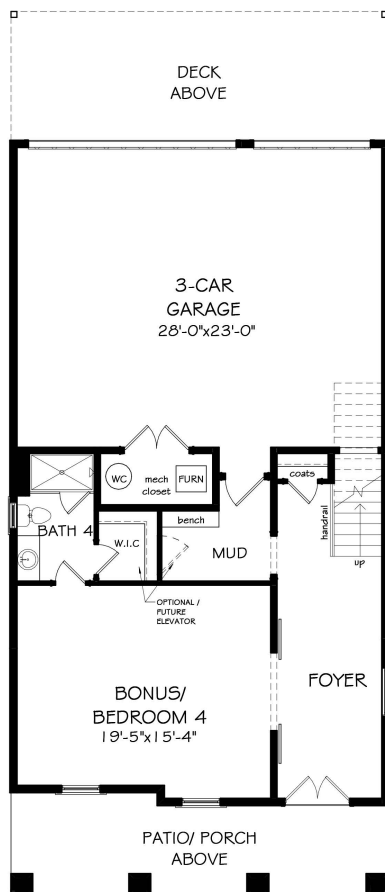
TERRACE LEVEL
