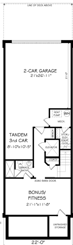
TERRACE LEVEL
